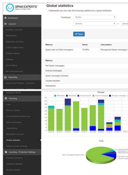
Global statistics
